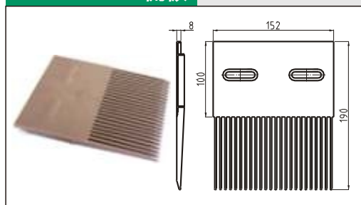
H3110T24梳板
