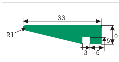
HDS471 瓶头托条
