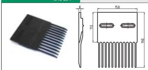
H5997T12梳板
