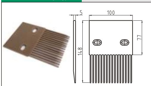
H100T16梳板
