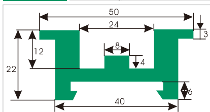
HDS432 槽型垫轨
