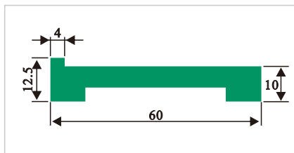
HDS058 L型盖型垫条
