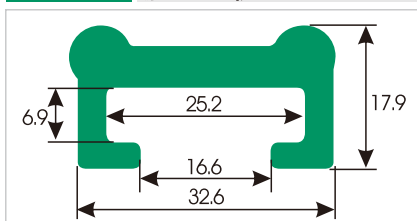
HDS440 槽型垫轨
