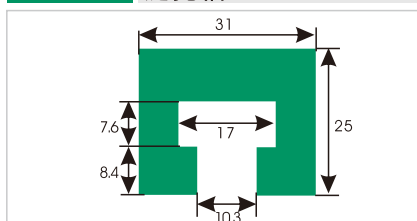
HDS463 链托槽A10
