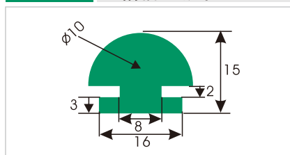
HDS439 圆帽槽型护栏
