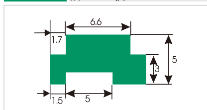
HDS430 槽型垫轨
